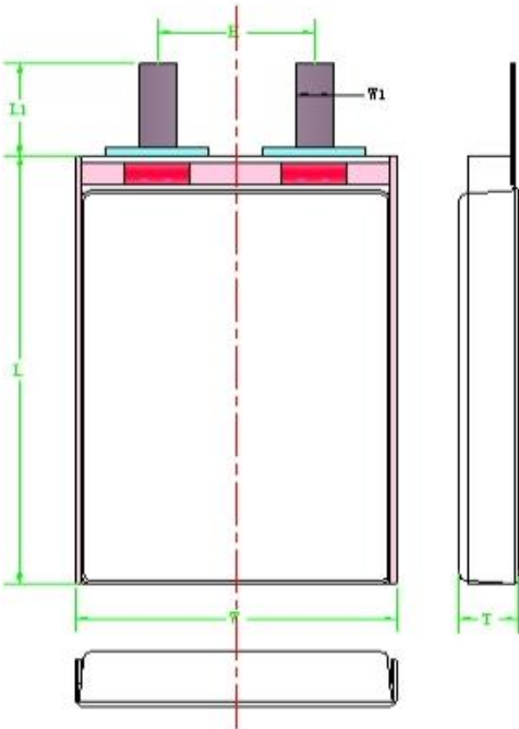
Cell: Max. 3.6mm (T) x Max. 14.0mm (W) x Max. 23.3mm (L)
