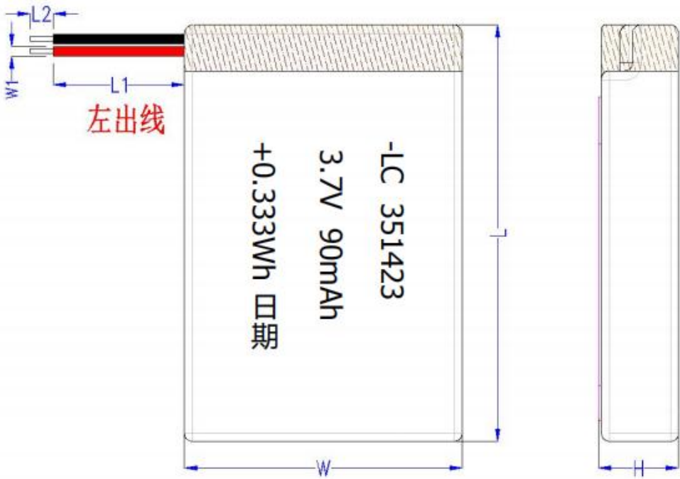
Battery: Max. 3.5mm (H) x Max. 14.0mm (W) x Max. 25.0mm (L)
